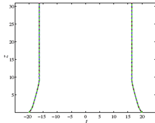
Fig. 6. An example of the collision between two identical slowly moving rhombic vortices, with relative velocity \Delta V = 2 and propagation constant \mu = 22 , as per Ref. [28].
