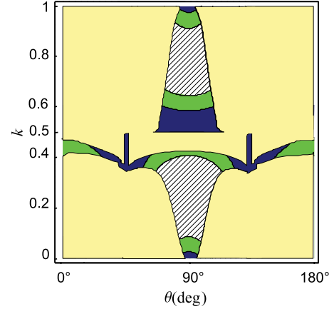
FIG. 5. (Color online) Evolution of the pulse duration in the (\theta, k) plane for L_2 = 19 m and L_3 = 24 m. In the hatched region, the duration is above 1 ps; in the green (dark gray) region, it is between 0.5 and 1 ps; and in the blue (black) region, below 0.5 ps. The yellow (light gray) regions have the same meaning as in Fig. 4.
