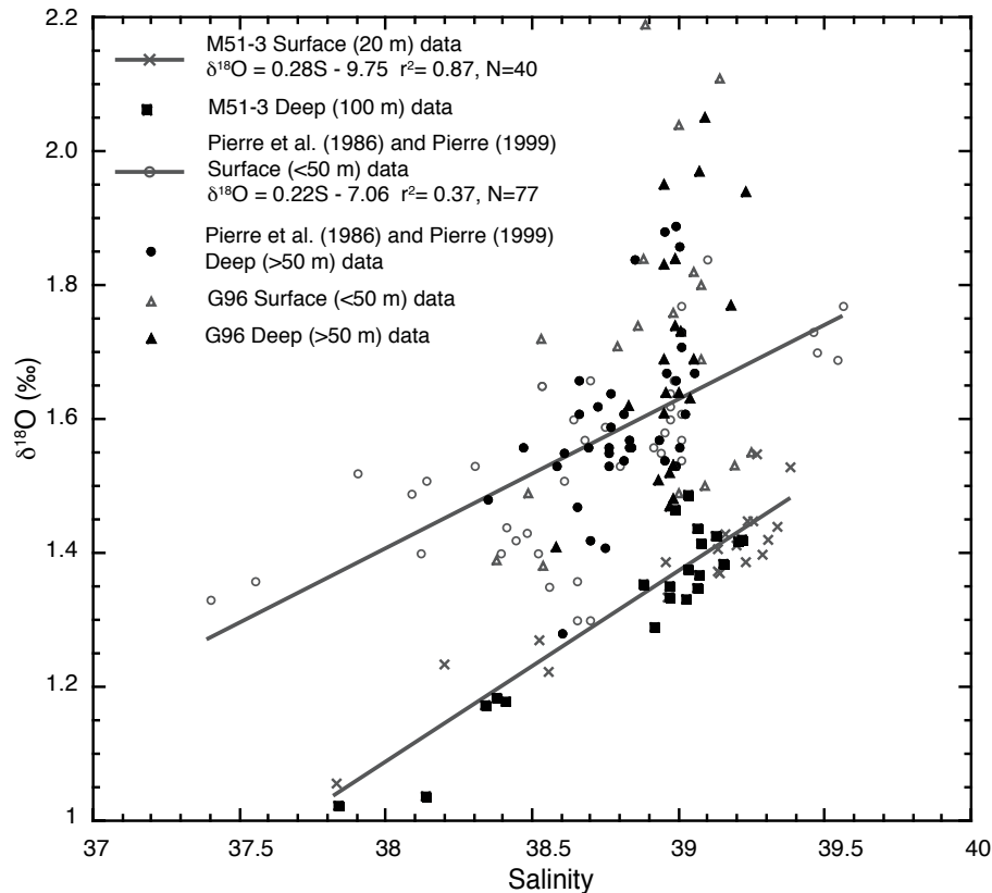
Fig. 4. Salinity: \delta^{18}\text{O} plot of M51-3 data (crosses and squares) compared with Pierre et al. (1986), Pierre (1999) (circles) and G96 (triangles). Grey data points denote surface water samples and black data points denote deep water samples.
