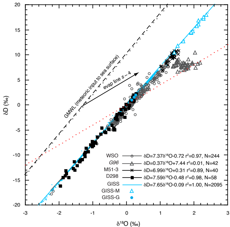
Fig. 1. The \delta^{18}\text{O}:\delta\text{D} mixing relationships, from top to bottom in the legend: the modern world surface (upper 250 m) ocean (WSO) (from Schmidt et al., 1999, originally reported by Duplessy, 1970; Weiss et al., 1979; Aharon and Chappell, 1986; Östlund et al., 1987; Yobbi, 1992; and Delaygue et al., 2001), the G96 Mediterranean dataset, the M51-3 Mediterranean dataset, the D298 Cape Farewell dataset, the complete GISS model data mixing relationship (Schmidt et al., 2007), the GISS model results from the Mediterranean (GISS-M) (Schmidt et al., 2007) and the GISS model results from the East Greenland region (GISS-G) (Schmidt et al., 2007). The GMWL and an example evaporation line are also plotted.
