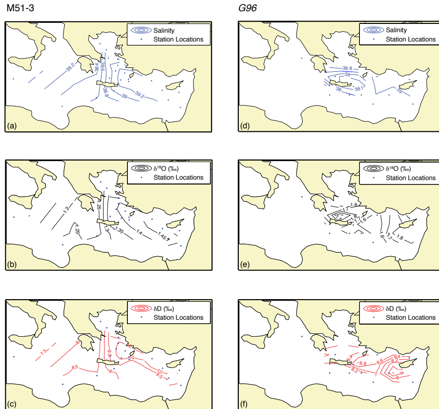
Fig. 3. Salinity, \delta^{18}\text{O} and \delta\text{D} and distribution maps of the M51-3 data (a, b, and c) and the G96 data (d, e and f).
