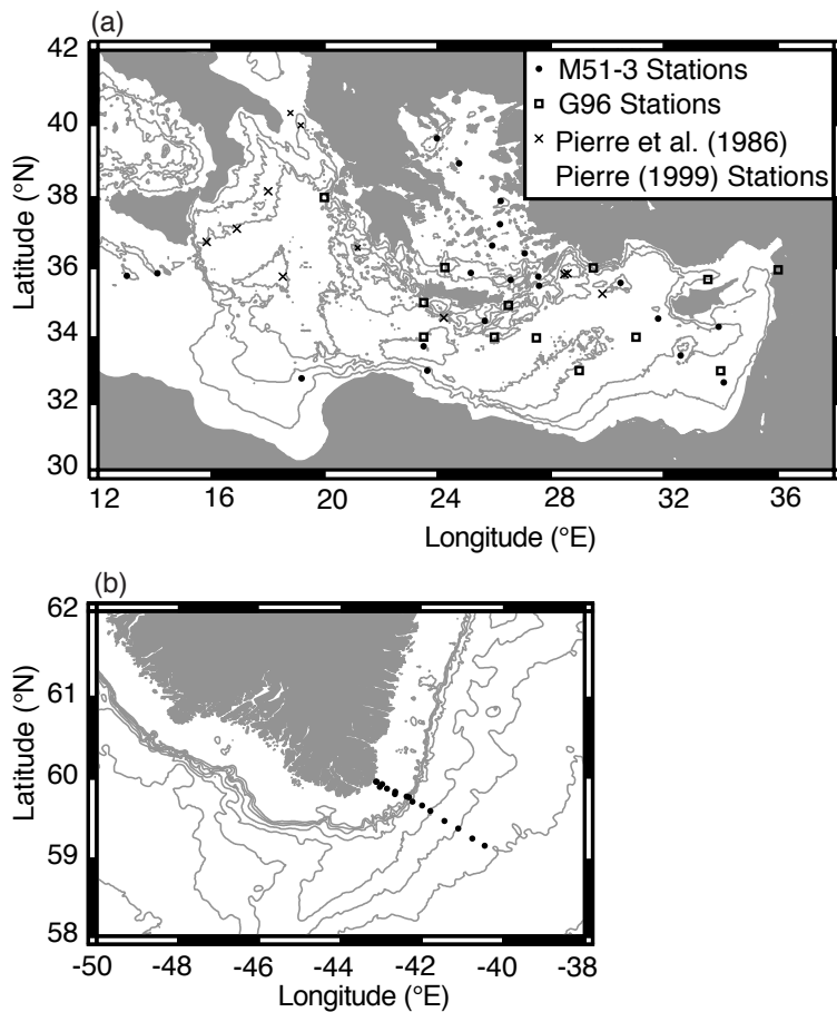
Fig. 2. Maps of the oxygen and hydrogen isotope data station locations for RV Meteor cruise M51-3, Pierre et al. (1986), Pierre (1999) and G96 (a) and the RRS Discovery cruise D298 (b).
