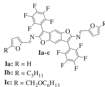
Fig. 1. Structure of the new conjugated derivatives 1a–c .
