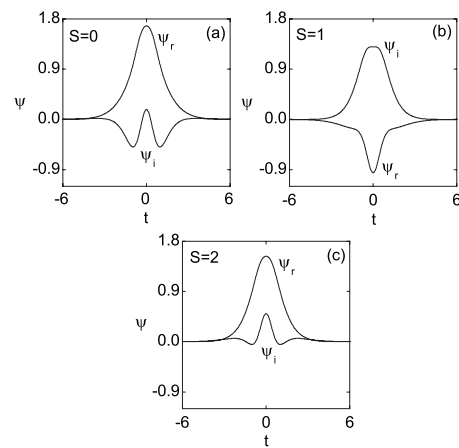
FIG. 3. The real and imaginary parts, \psi_r and \psi_i , of the temporal shapes for S=0 (a), S=1 (b), and S=2 (c). The parameters are as in Fig. 1.
