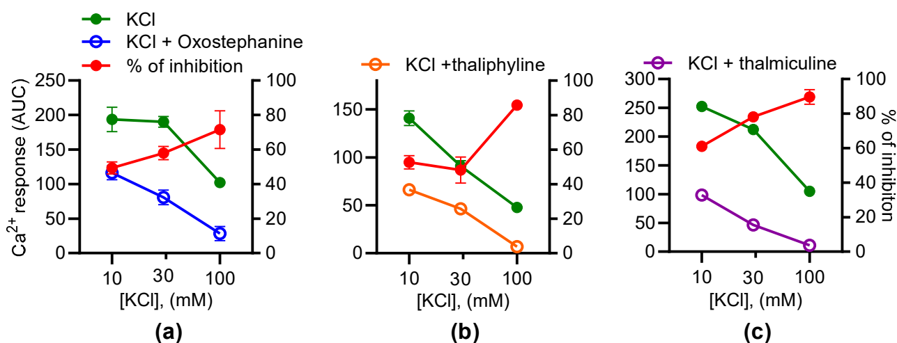
Figure 7. The inhibitory effects of oxostephanine, thaliphylline, and thalamiculine versus the KCl concentrations. The effects of 10 \mu\text{M} of oxostephanine (a), thaliphylline (b), and thalamiculine (c) were evaluated on \text{Ca}^{2+} responses induced by increasing concentrations of KCl (10, 30, and 100 mM). Left y axis: AUC were determined from kinetics of the Fura-2 emission fluorescence ratio. Right axis: the inhibition was calculated as a ratio of AUC of kinetic traces in the presence and absence of IAs in %. Data are mean \pm SEM ( n = 3 ).
